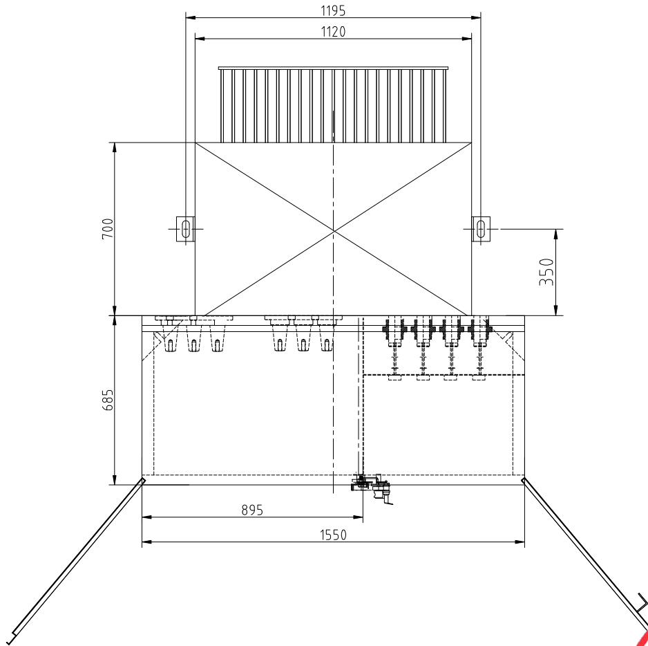
TOP VIEW OF BASE & HV-LV COMPARTMENT
